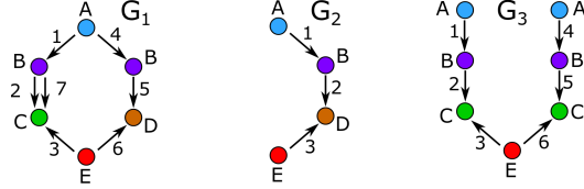
Figure 3: Temporal graphs: (1) G_2 is a temporal subgraph of G_1 ( G_2 \subseteq_t G_1 ); and (2) G_1 and G_2 are T-connected, while G_3 is non T-connected.
