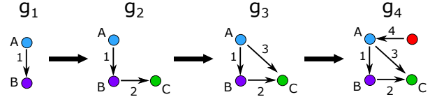
Figure 4: An example of consecutive growth
